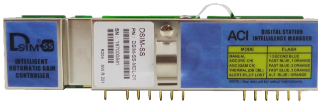
DSIM-SS 01 (W/O EQ) For Cisco®/Scientific Atlanta® System Amplifier II & III
