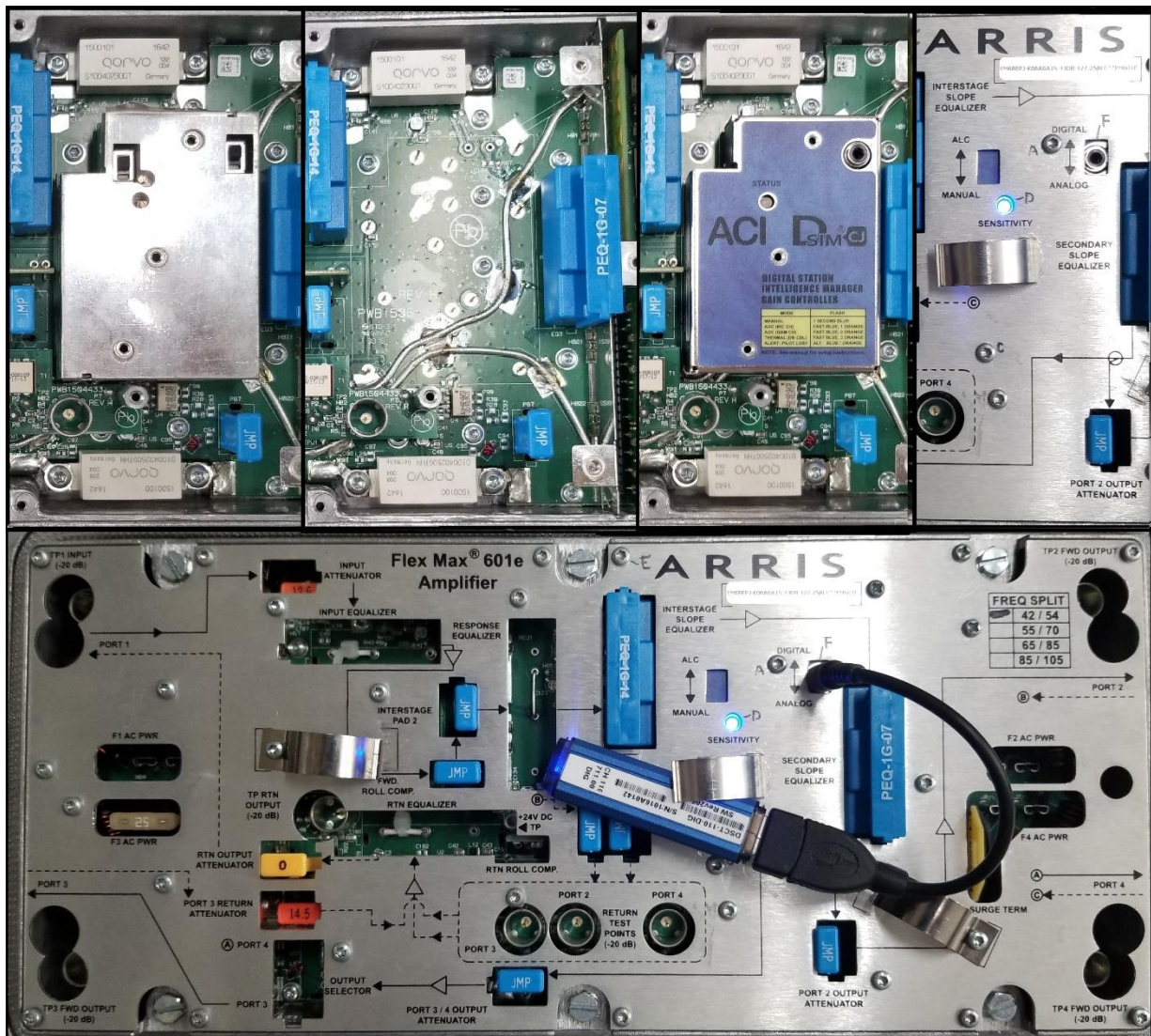
Controller Connection to DSIM
