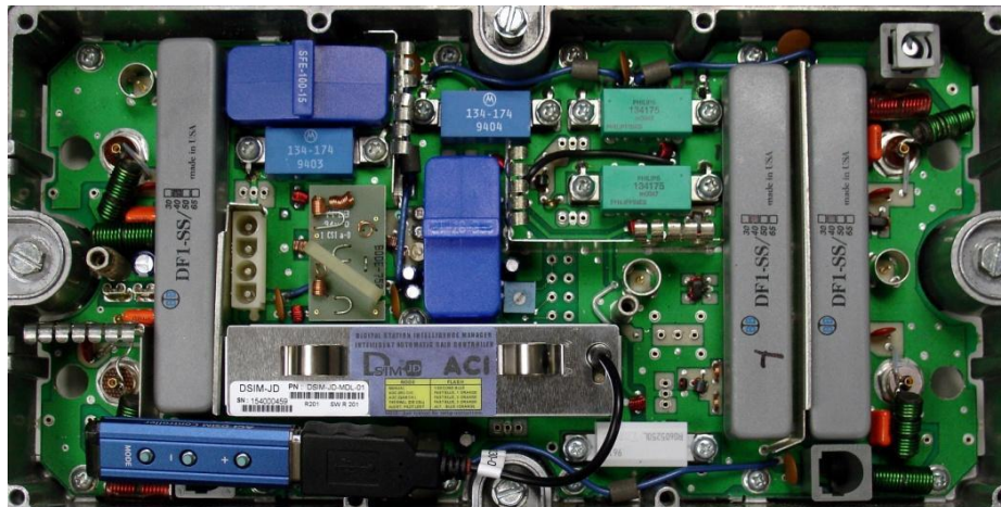
Controller Connection to DSIM (Shown with faceplate cover removed for clarity)
